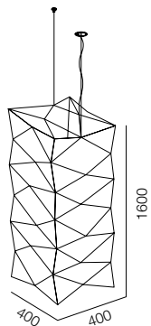
SUPREME SOZVEZDIE LINE 160
