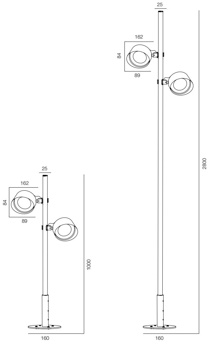
GARDEN PIN 25 1000
