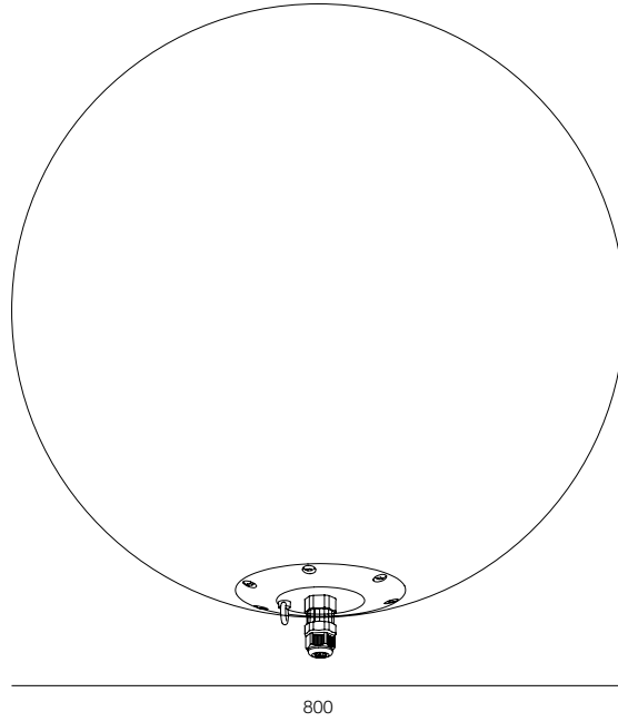
GARDEN FLOAT 800
