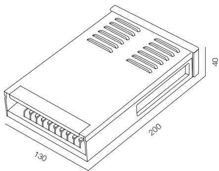
ERPF 400-24/48V
