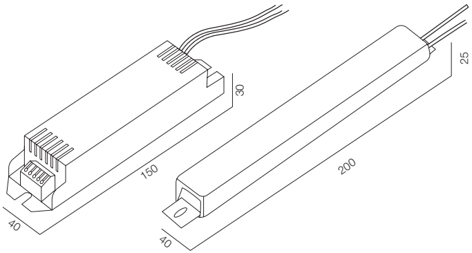
EMERGENCY POWER 40W
