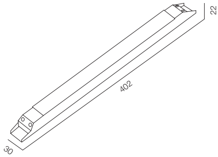
POWER SLD 200-48V DALI 0,1%
