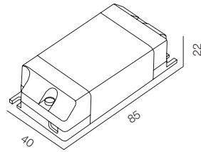
DIM TRIAC 220V SD
