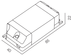
DIM TRIAC 220V SD
