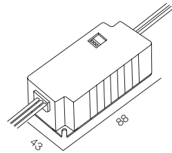
DRIVER DALI DIM 0,1% 40W 850-1200MA
