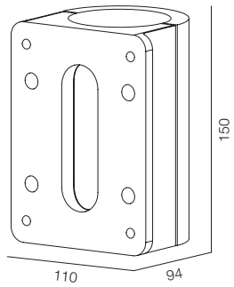
POLE 68 BRACKET CAMERA
