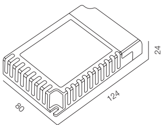
DIM DALI DRIVER 50W
