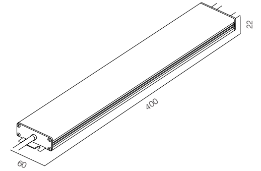
POWER SPL (KG) 400W 48V IP67 DALI
