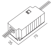
DRIVER DALI DIM 0,1% 10W 350-700MA
