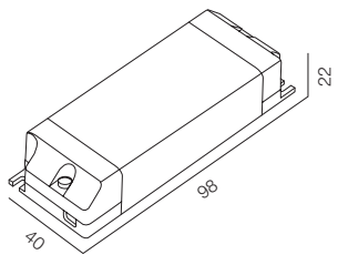
DIM DALI DRIVER 20W
